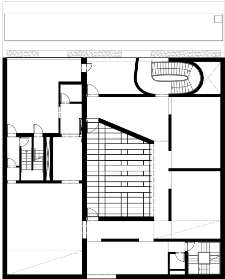
LEVEL 3 [+56'-0"]
