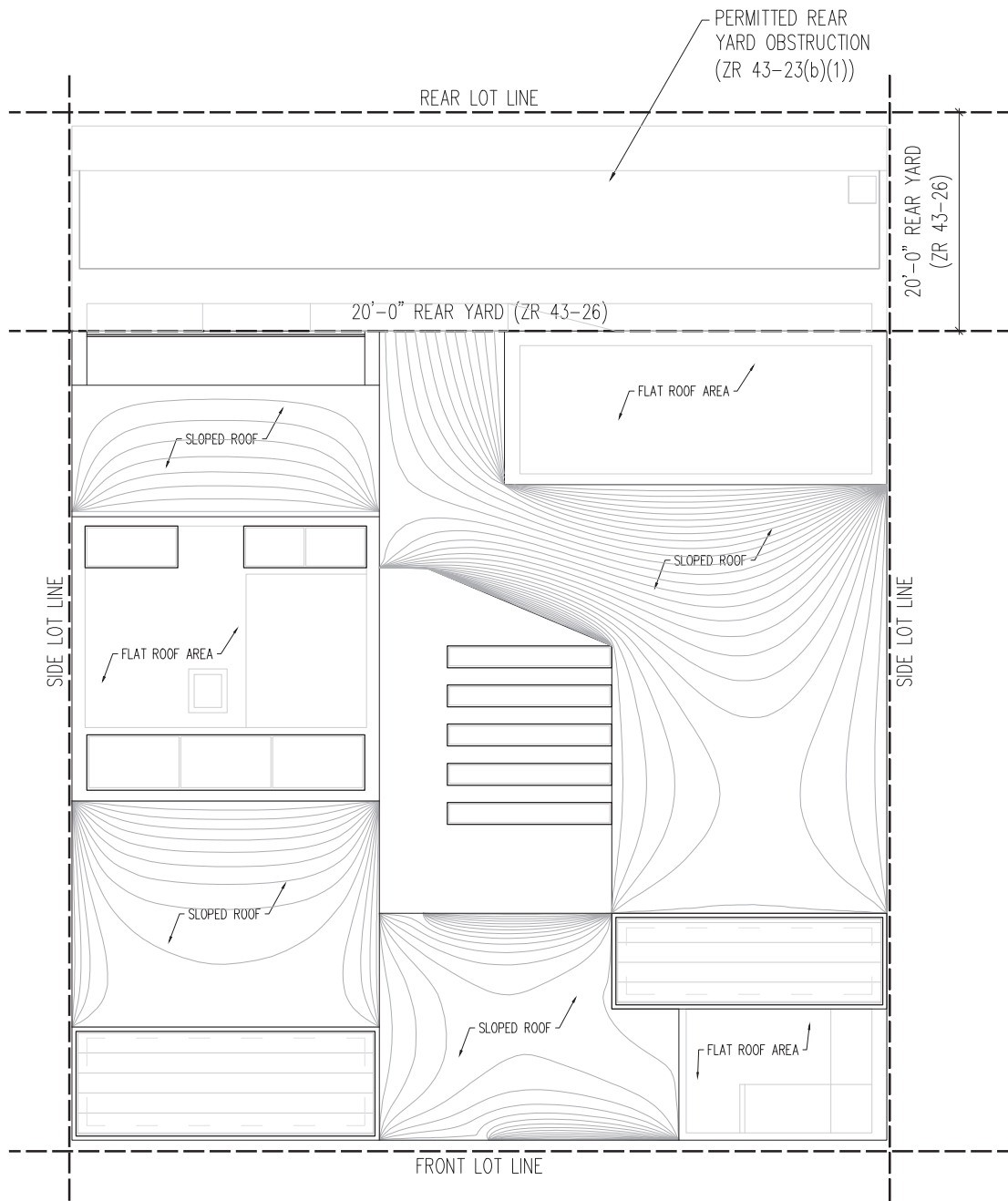
ROOF PLAN
