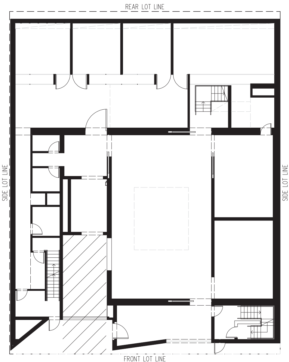
GROUND LEVEL [+26'-6"]
