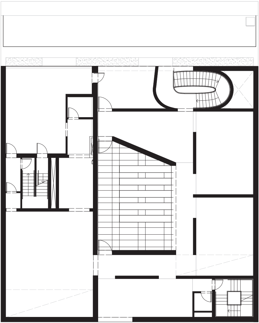
LEVEL 3 [+56'-0"]
