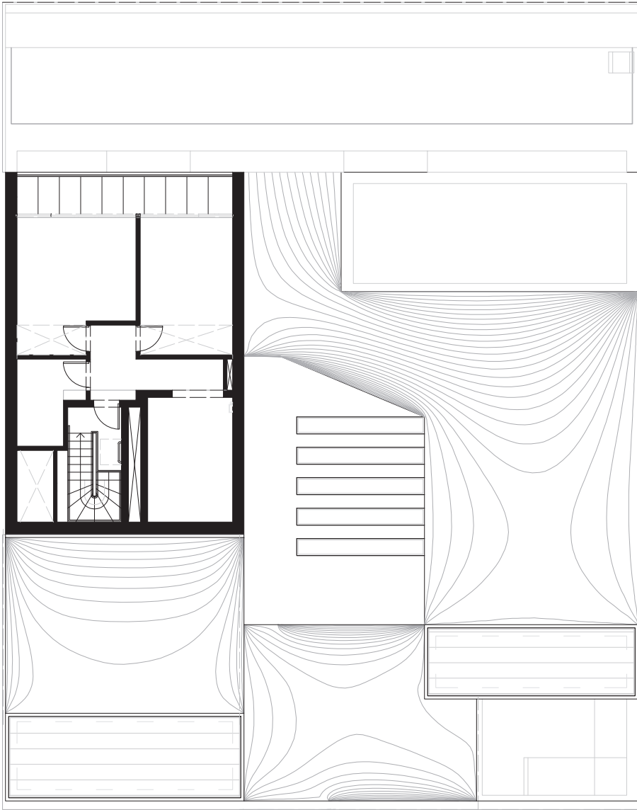
LEVEL 4 [+68'-0"]
