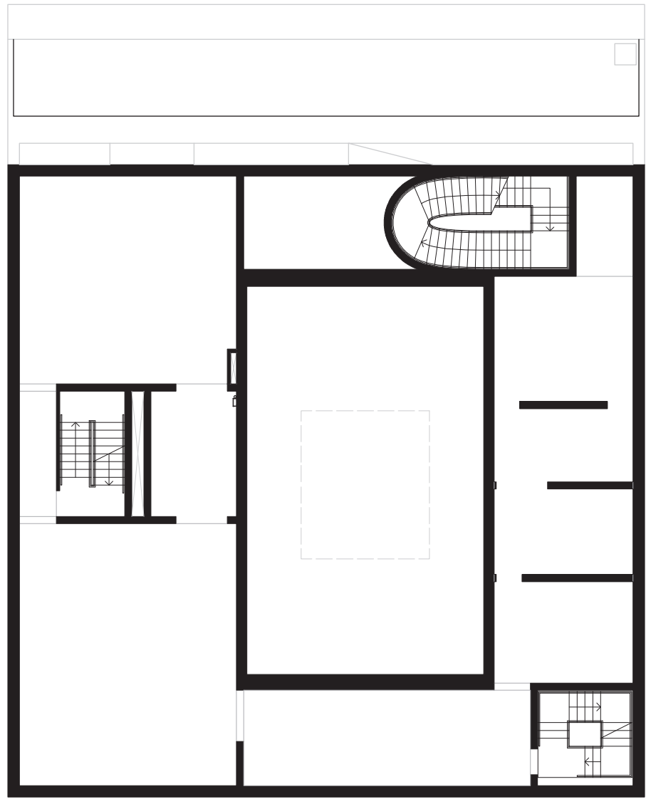
LEVEL 2 [+43'-6"]
