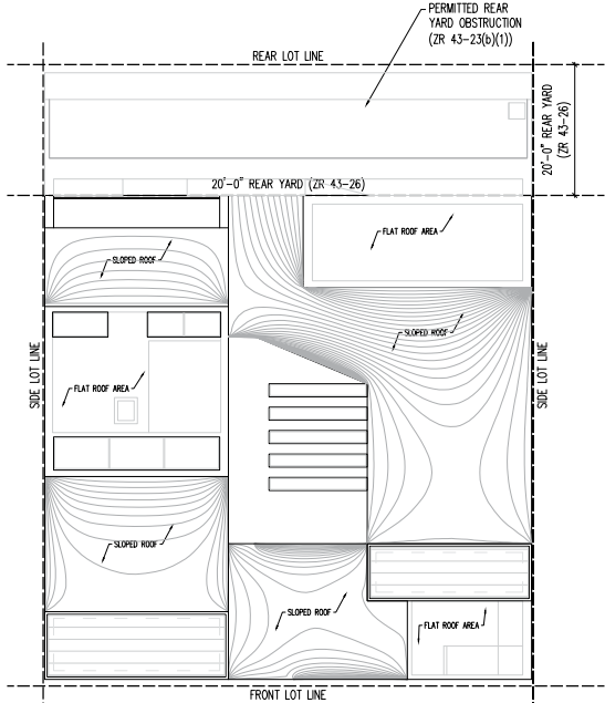
ROOF PLAN
