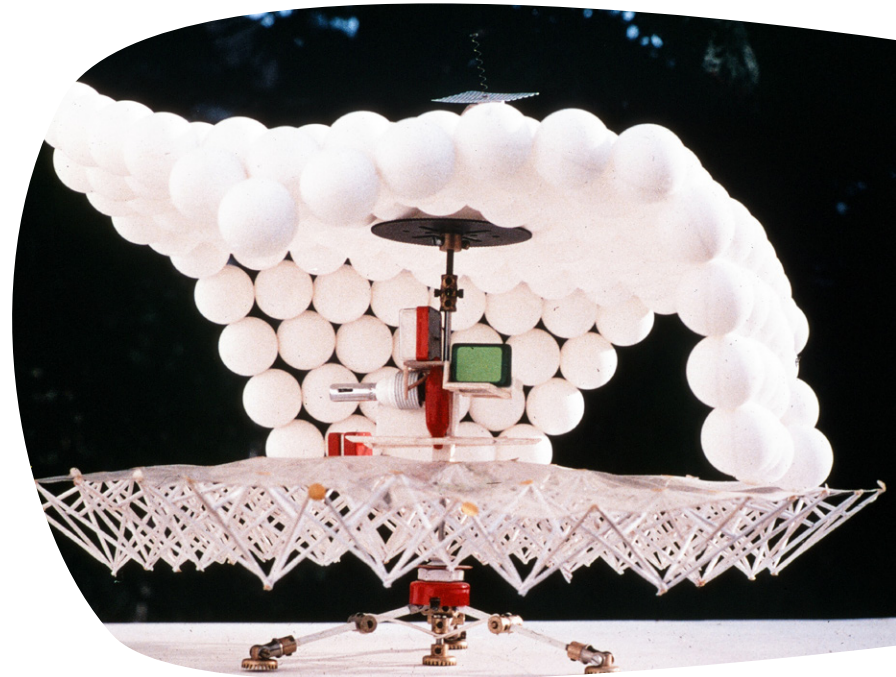
This model—a lightweight structure, comprised of a dual-walled pneumatic mat (indicated here by Ping-Pong balls)—was designed by Mike Davies as the off-the-grid Energy House (1970) that could be easily packed up into a van, driven, and deployed just about anywhere.
